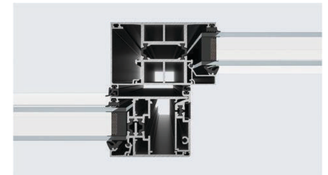
90 Enforced Mullion
