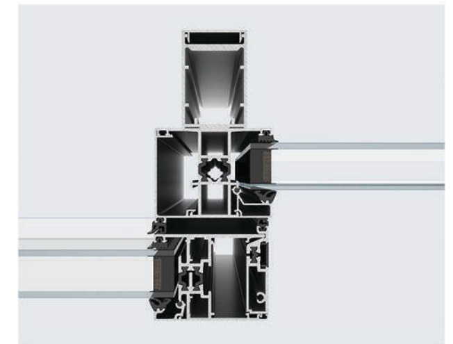
70 Standard Mullion + 40 Enforced
