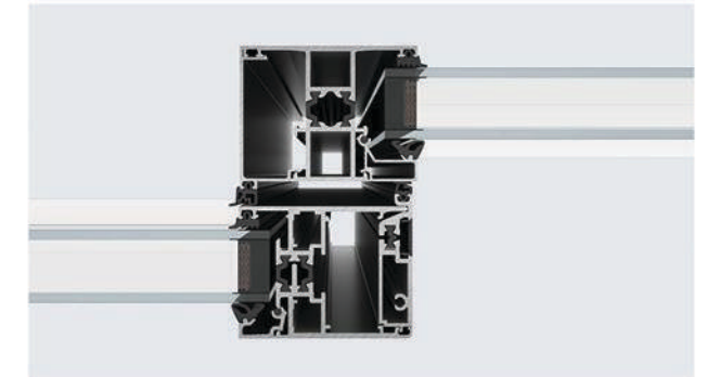
70 Standard Mullion
