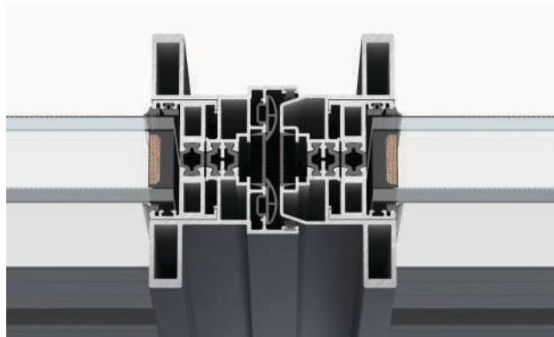
Closing treatment of double sash
