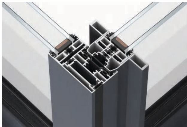
Corner closing treatment
