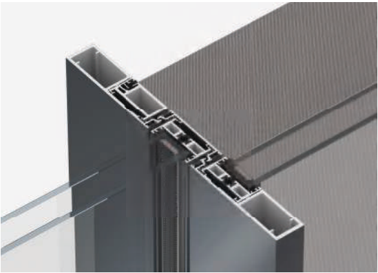
32mm enforced overlap(Three-tracks with screen)
